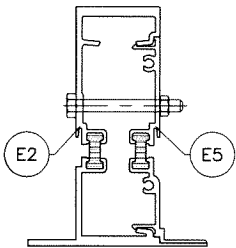
MULLION 'M1'
